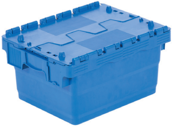
HP-4321-MK En/W Boy/L Yük/H Dış / Ext 300 x 400 x 210 mm İç / Int 265 x 340 x 190 mm
