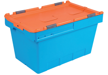
HX-5326-MK En/W Boy/L Yük/H Dış / Ext 300 x 490 x 275 mm İç / Int 257 x 430 x 255 mm
