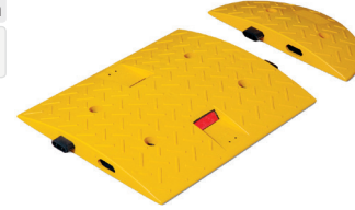
12106 YK En/W Boy/L Yüksek/H 400 x 500 x 40 mm Ağırlık / Weight 6,50 Kg Material Kauçuk şase PVC Compoud / Rubber
